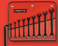
JSCR-9S PROTO® 9 PIECE BLACK CHROME NON-REVERSIBLE COMBINATION RATCHETING WRENCH SET - SPLINE
